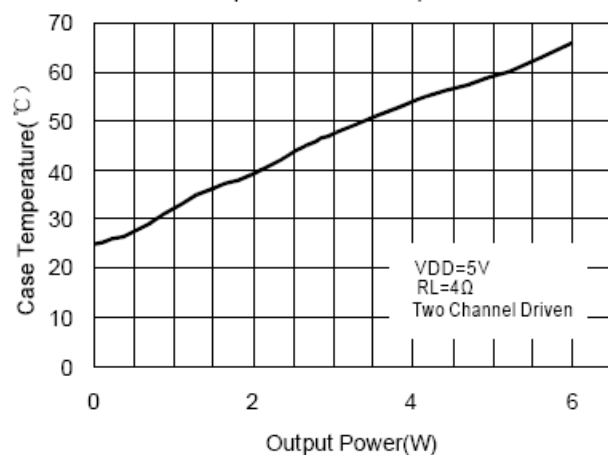
11. Case Temperature vs Output Power
