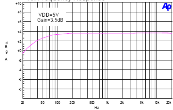
16. Frequency Response
