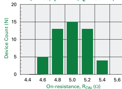
Typical On-resistance Distribution (N = 50, I_F = 2 mA, I_L = 150 mA)
