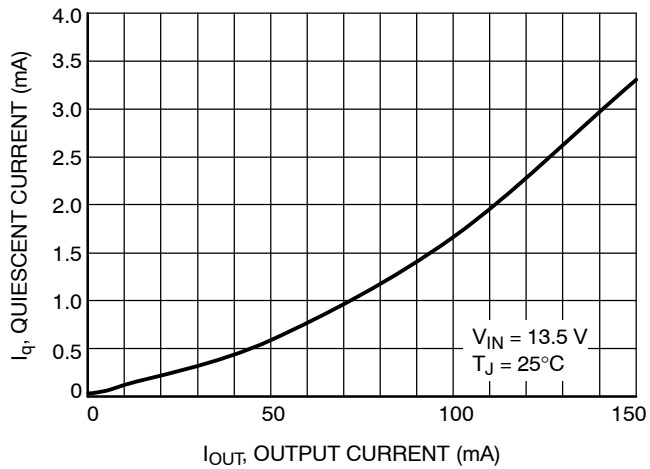
Figure 16. Quiescent Current vs. Output Current (3.3 V Version) (High Load)
