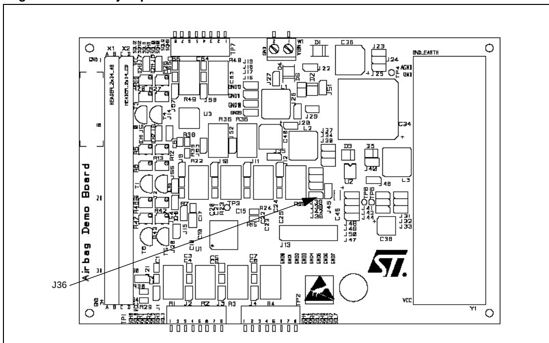
Figure 10. Reset jumper
