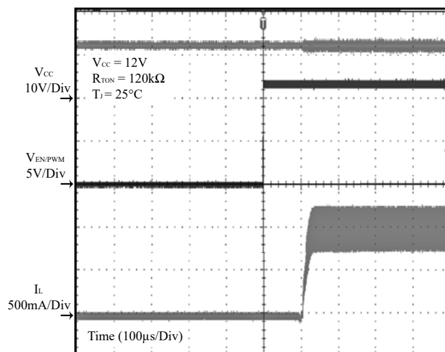
Figure 31 EN/PWM Enable
