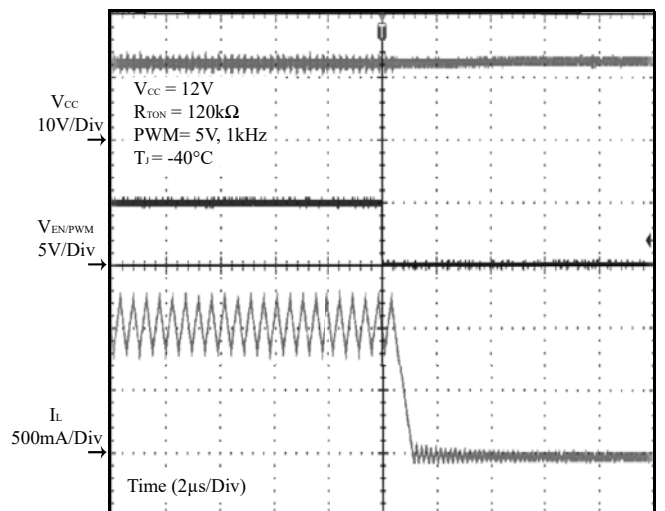
Figure 25 PWM Off
