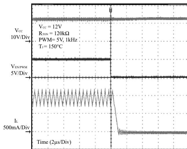
Figure 29 PWM Off
