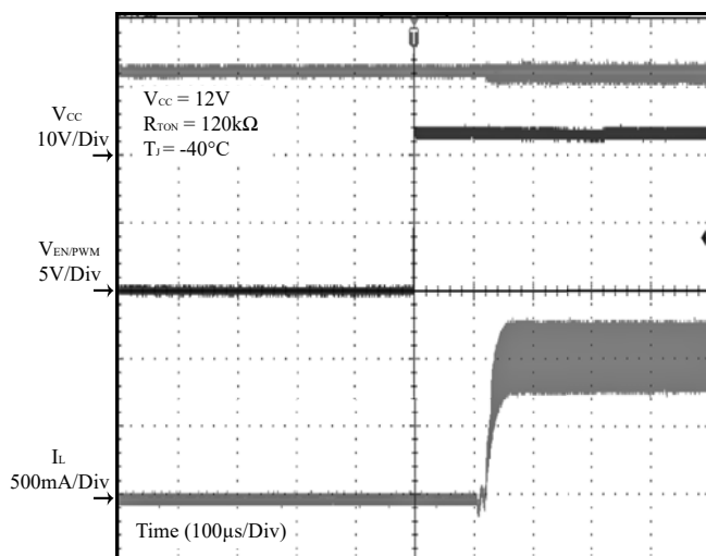
Figure 30 EN/PWM Enable
