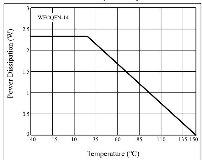
Figure 51 Dissipation Curve
