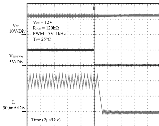
Figure 27 PWM Off
