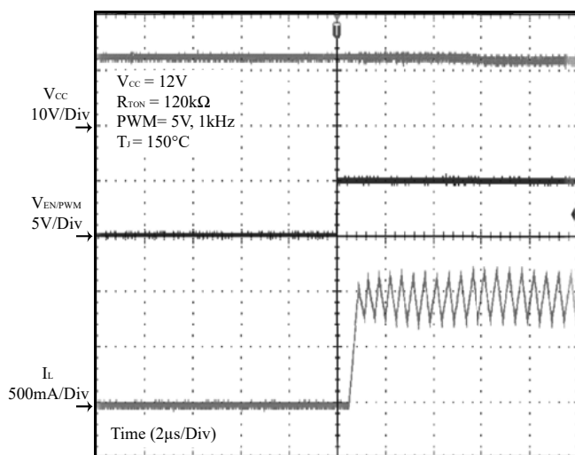
Figure 28 PWM On
