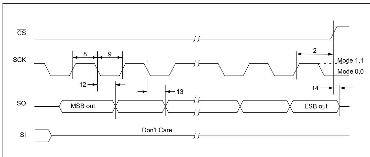
FIGURE 1-6: SPI Output Timing.
