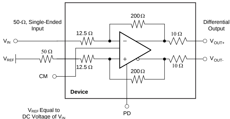
Figure 54. Single-Ended Input to Differential Output Amplifier
