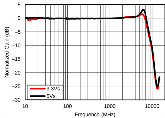
Figure 2. Frequency Response Differential Input
