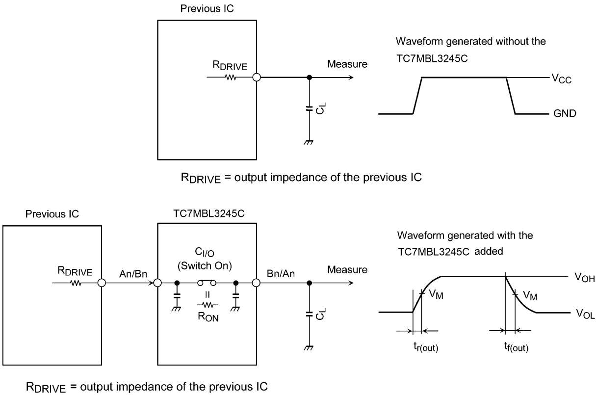
Fig. 12.1 Calculation Circuit
