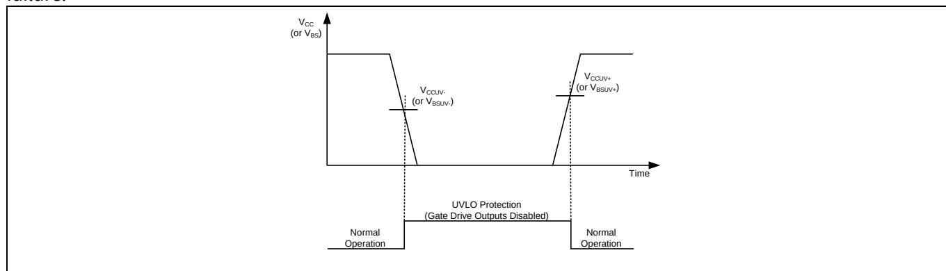
Figure 12 UVLO protection
