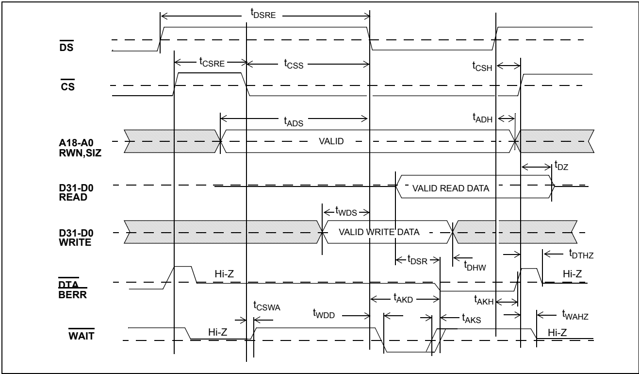
Figure 15 - Microprocessor Bus Interface Timing
