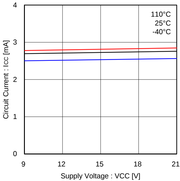
Figure 9. Circuit current
