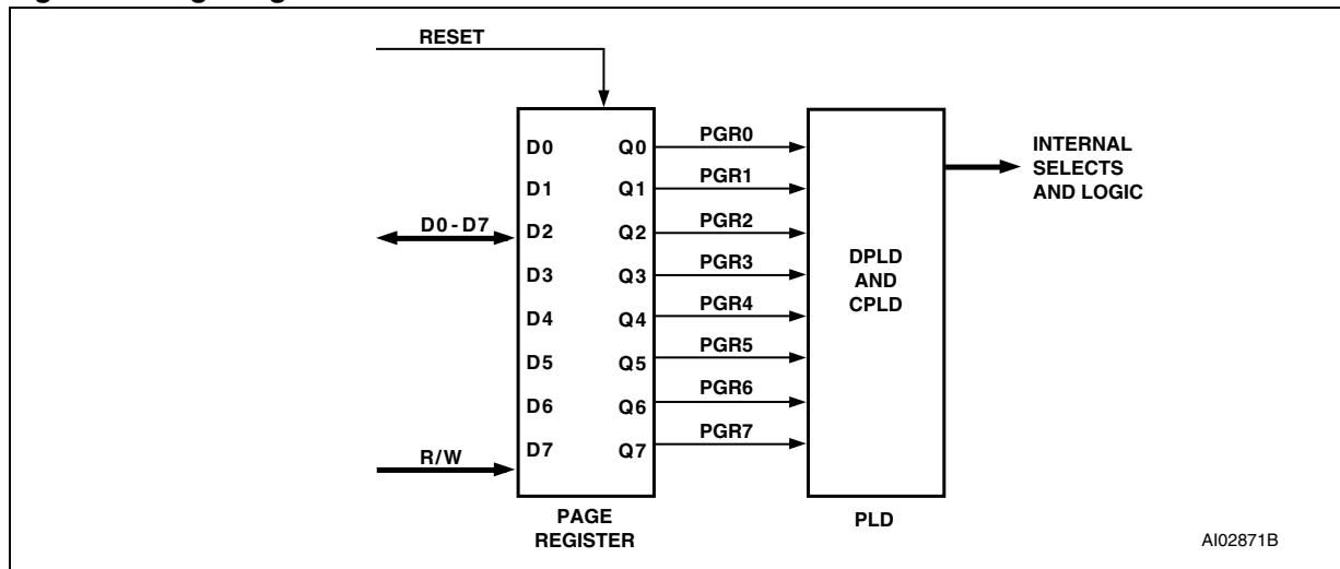
Figure 12. Page Register
