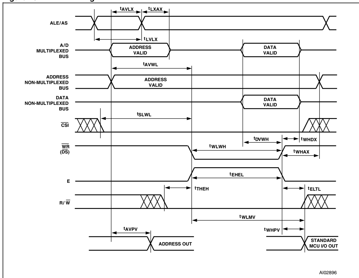
Figure 46. WRITE Timing
