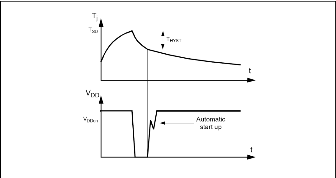
Figure 13. Thermal shutdown
