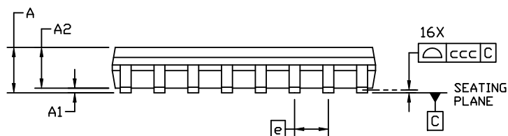
Figure 6.2. 16-pin Small Outline Integrated Circuit (SOIC) Package
