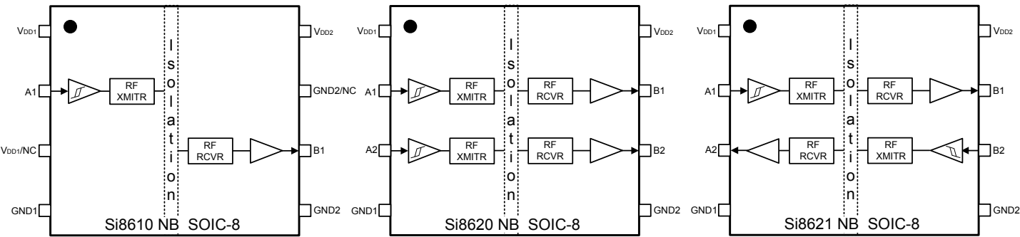
Figure 5.1. Si861x/2x Narrow Body SOIC-8 Pin Descriptions
