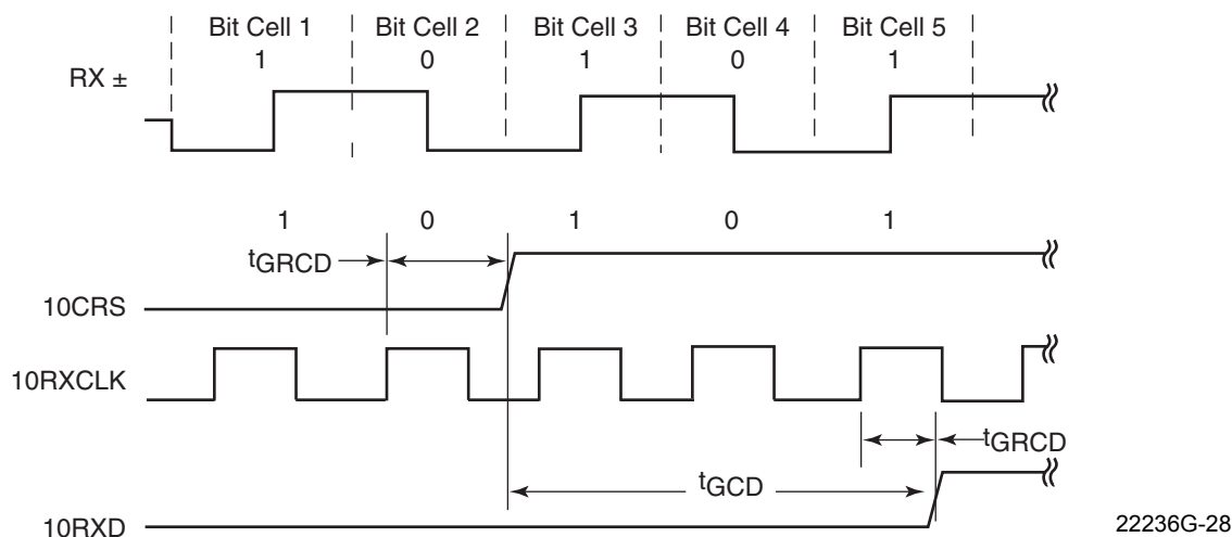
Figure 26. GPSI Receive Timing - Start of Reception
