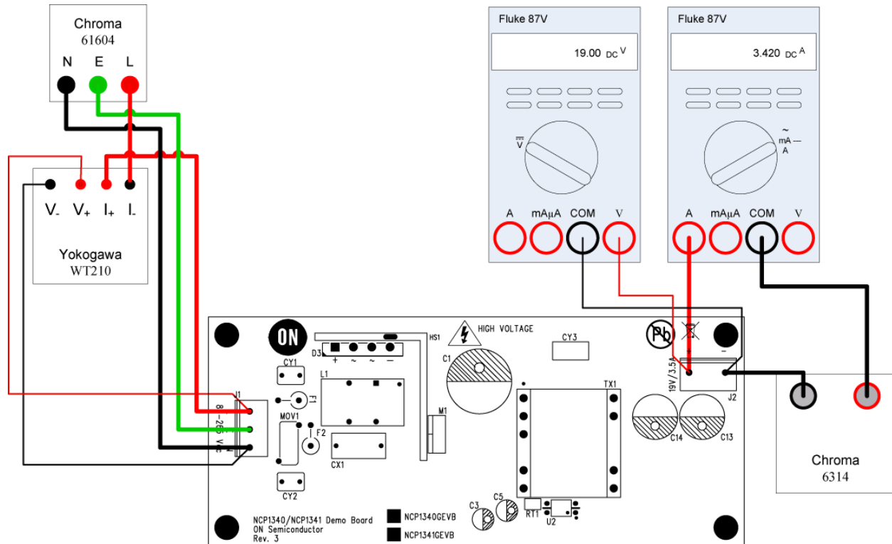
Figure 1: Test Setup
