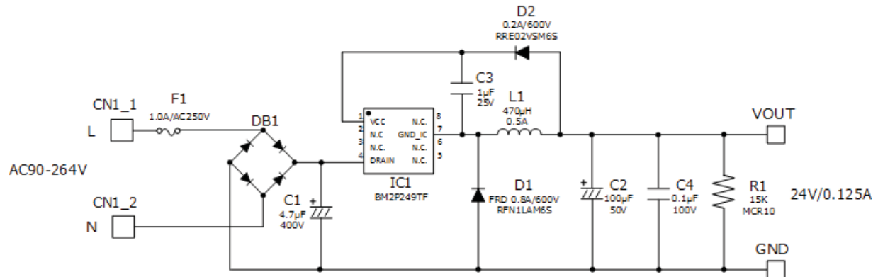
Figure 23. BM2P249TF-EVK-001 Schematics
