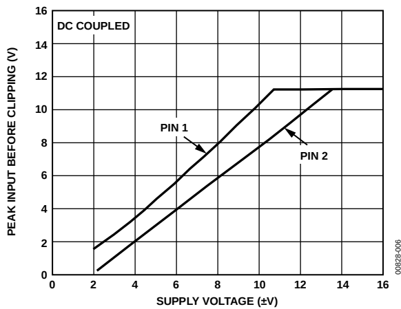
Figure 6. Maximum Input Level vs. Supply Voltage
