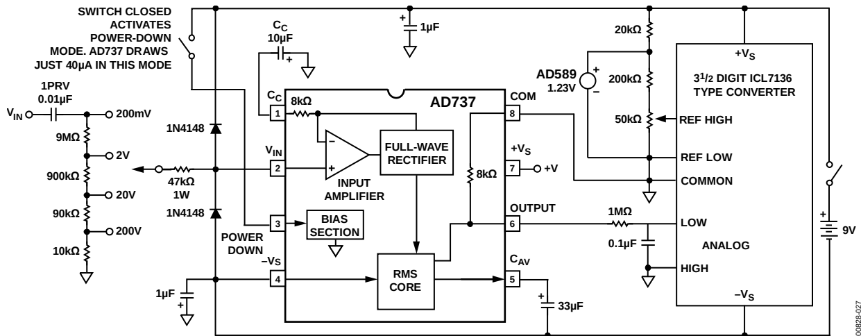
Figure 28. 3 1/2 Digit DVM Circuit
