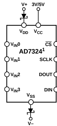
Figure 54. Schottky Diode Connection
