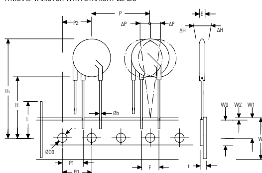
iTMOV® VARISTOR WITH STRAIGHT LEADS
