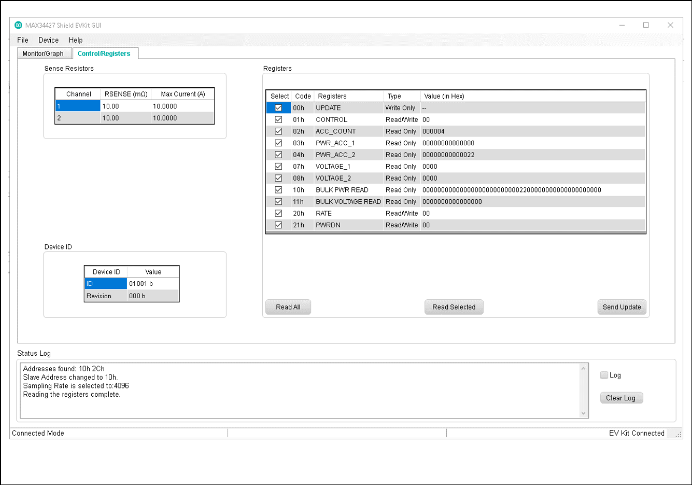
Figure 3. MAX34427 Shield EV Kit GUI—Control/Registers Tab
