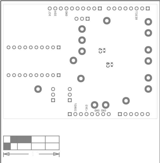
MAX34427 EV Kit PCB Layout—Bottom Silkscreen
