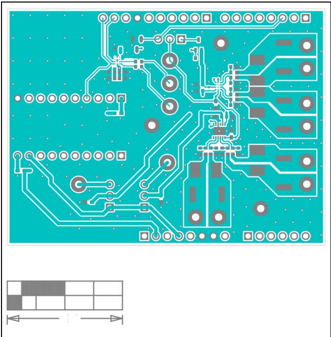
MAX34427 EV Kit PCB Layout—Top Layer
