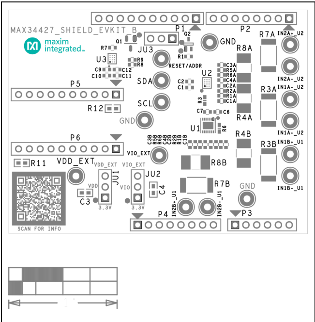
MAX34427 EV Kit PCB Layout—Top Silkscreen
