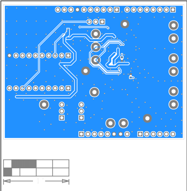
MAX34427 EV Kit PCB Layout—Bottom Layer
