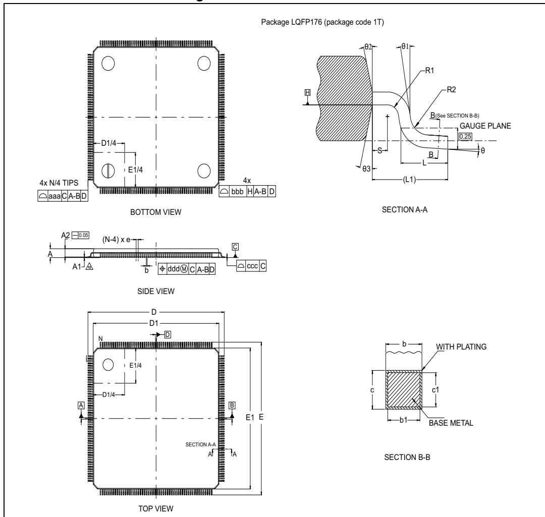
Figure 89. LQFP176 - Outline
