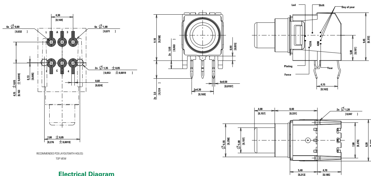
K5V 1 THT 3.5mm Drawing and Dimensions (mm)
