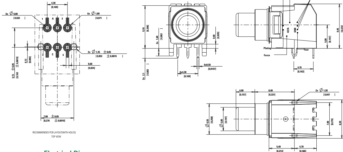
K5V 1 THT 2.1mm Drawing and Dimensions (mm)
