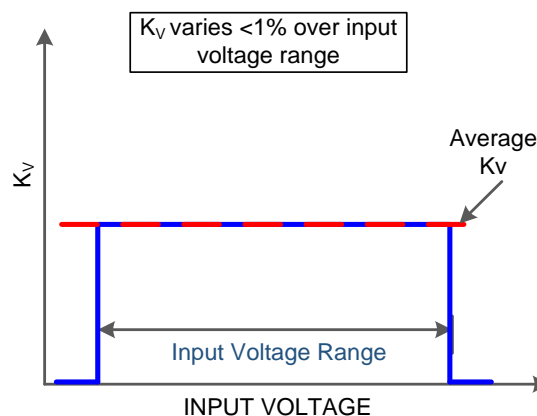
Figure 50. Typical SiTime K_V Variation
