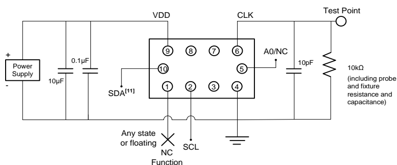
Figure 13. Clipped Sinewave Test Circuit (I²C Control), DCTCXO mode for AC and DC Measurements
