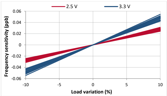
Figure 28. Load sensitivity
