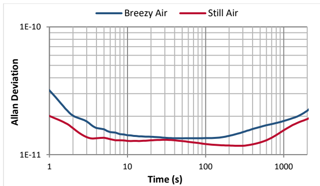
Figure 20. ADEV (0.1 Hz loop bandwidth) [14]
