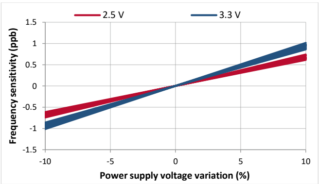
Figure 29. VDD sensitivity
