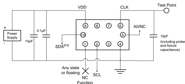
Figure 12. LVCMOS Test Circuit (I²C Control), DCTCXO mode for AC and DC Measurements
