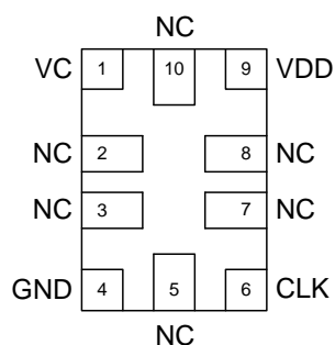
Figure 4. VCTCXO
