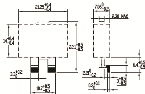
PQ2006-1R0-30-G | 1.0 μH
