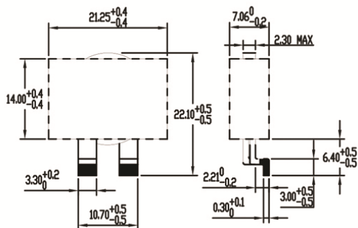
PQ2007-4R4-15-G | 4.4 μH
