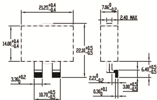
PQ2613-1R0-80-G | 1.0 μH
