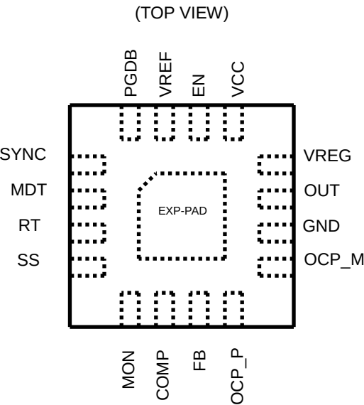
Figure 2. Pin Configuration
