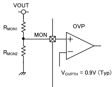
Figure 10. Circuit Diagram of OVP Function Setting Method
