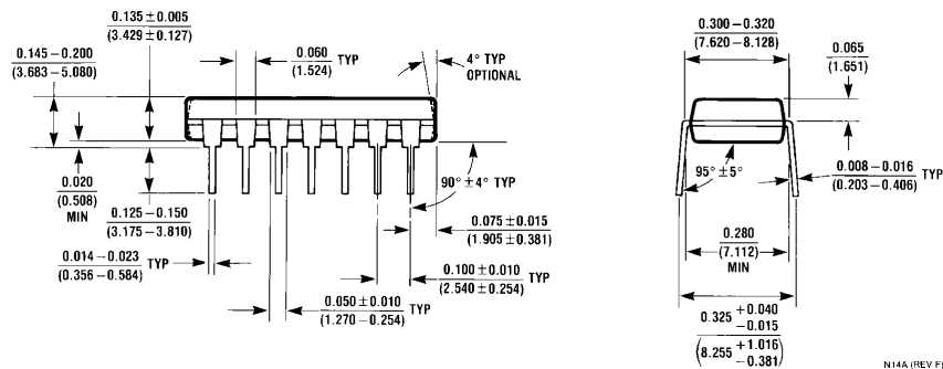
Dual-In-Line Package (N) Order Number LM322N NS Package Number N14A
