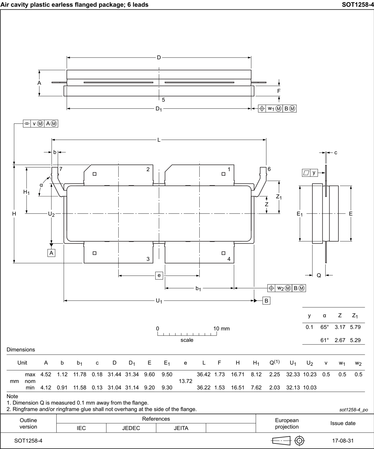
Fig 12. Package outline SOT1258-4
