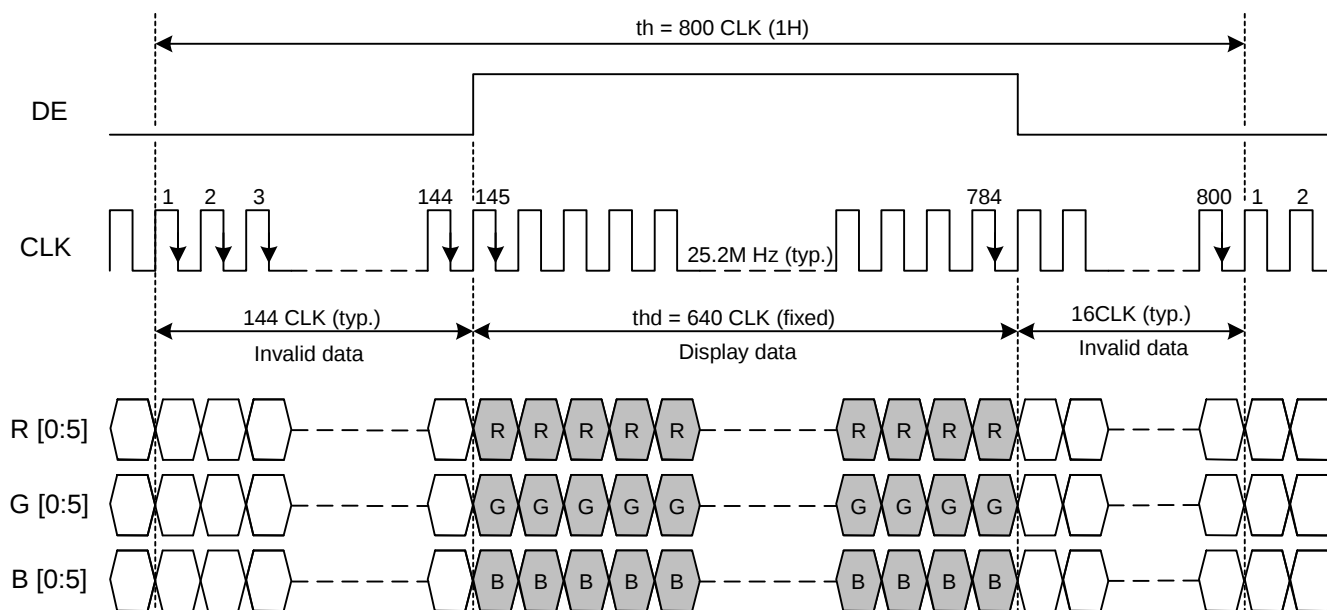
Fig. 9.3 Horizontal Timing of DE Mode
