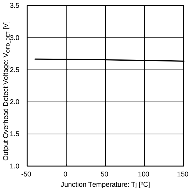
Figure 45. Output Overhead Detect Voltage vs Junction Temperature
