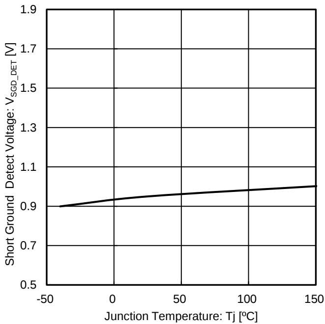
Figure 47. Short Ground Detect Voltage vs Junction Temperature
