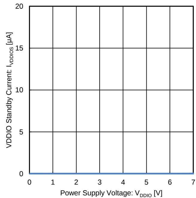
Figure 10. VDDIO Standby Current vs Power Supply Voltage
