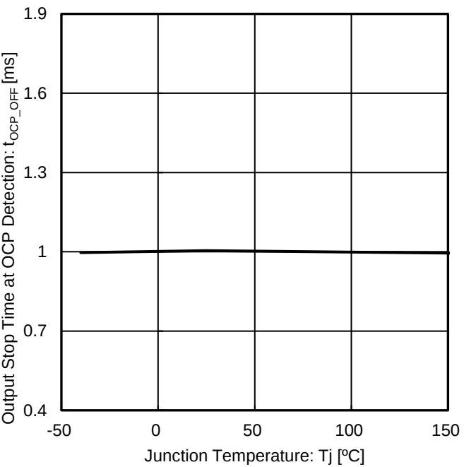
Figure 41. Output Stop Time at OCP Detection vs Junction Temperature
