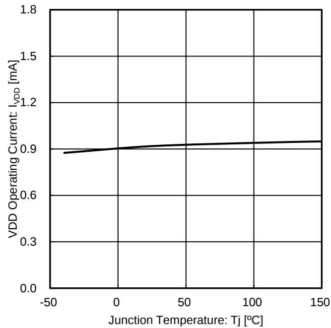
Figure 13. VDD Operating Current vs Junction Temperature
