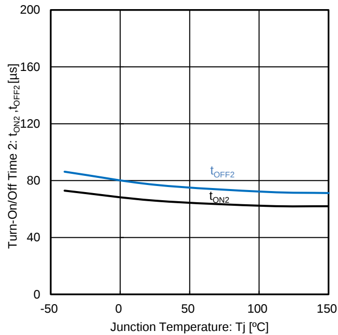
Figure 33. Turn-On/Off Time 2 vs Junction Temperature
