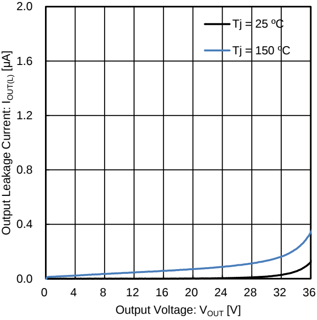
Figure 25. Output Leakage Current vs Output Voltage
