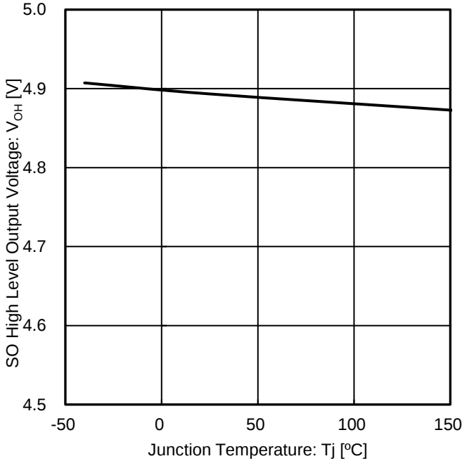
Figure 21. SO High Level Output Voltage vs Junction Temperature
