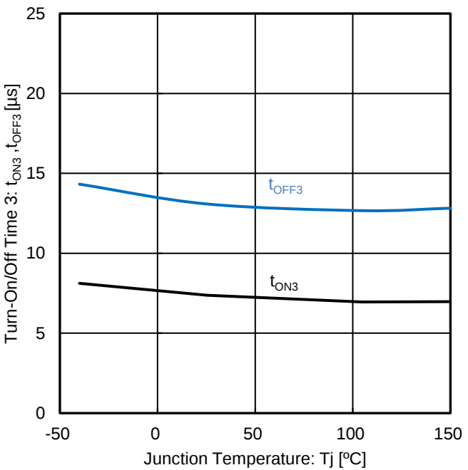
Figure 37. Turn-On/Off Time 3 vs Junction Temperature
