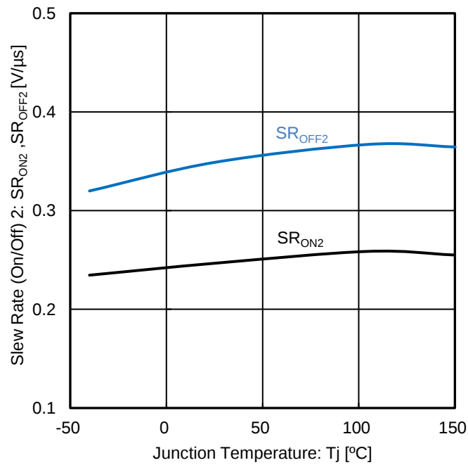
Figure 35. Slew Rate (On/Off) 2 vs Junction Temperature
