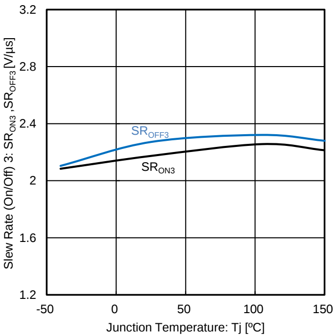
Figure 39. Slew Rate (On/Off) 3 vs Junction Temperature
