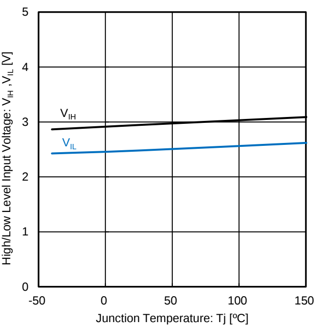
Figure 17. High/Low Level Input Voltage vs Junction Temperature
