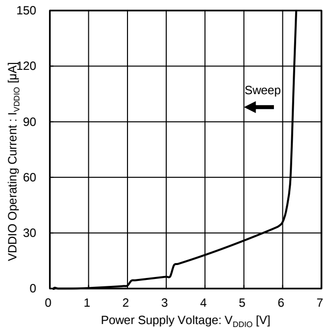
Figure 14. VDDIO Operating Current vs Power Supply Voltage
