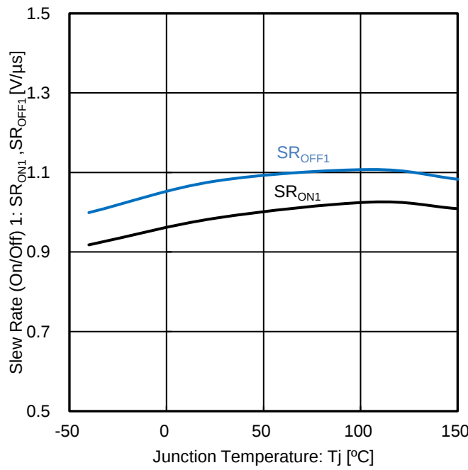
Figure 31. Slew Rate (On/Off) 1 vs Junction Temperature
