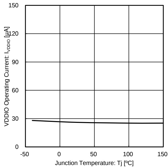
Figure 15. VDDIO Operating Current vs Junction Temperature
