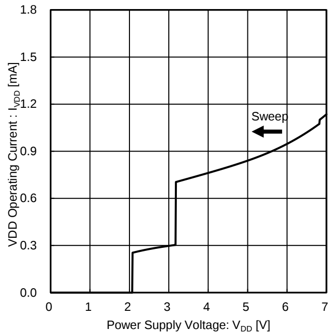
Figure 12. VDD Operating Current vs Power Supply Voltage
