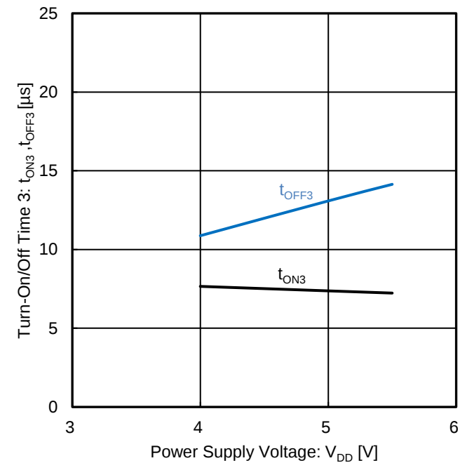
Figure 36. Turn-On/Off Time 3 vs Power Supply Voltage
