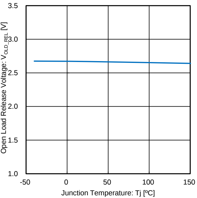
Figure 43. Open Load Release Voltage vs Junction Temperature
