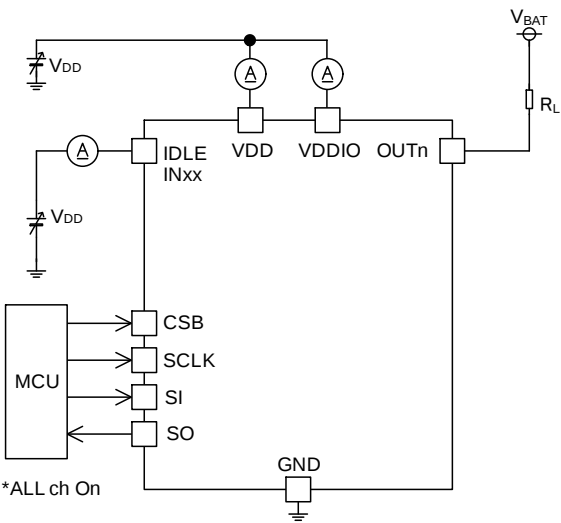
Figure 52. VDD Operating Current VDDIO Operating Current VDD Power On Reset Voltage VDDIO Power On Reset Voltage Thermal Shutdown Detect Temperature Thermal Shutdown Hysteresis Temperature
