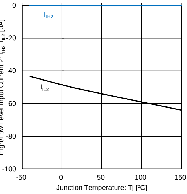
Figure 19. High/Low Level Input Current 2 vs Junction Temperature
