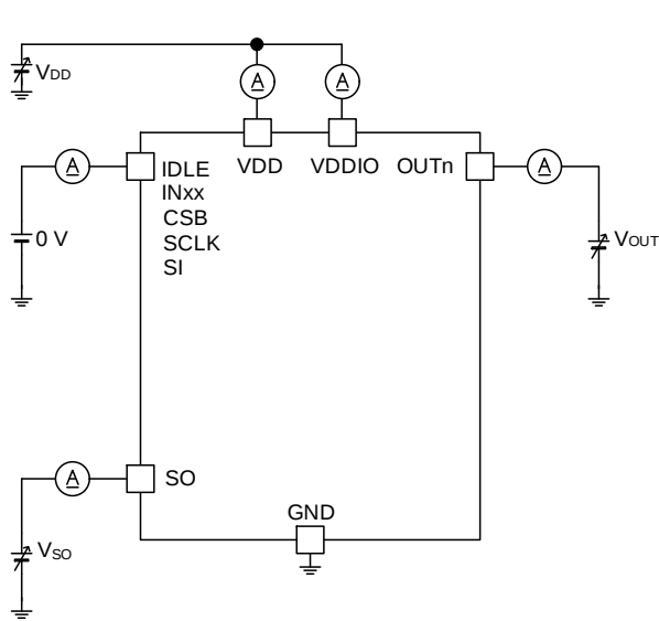
Figure 51. VDD Standby Current VDDIO Standby Current Low Level Input Current 1, 2 Output Leakage Current Serial Out Output Leakage Current
