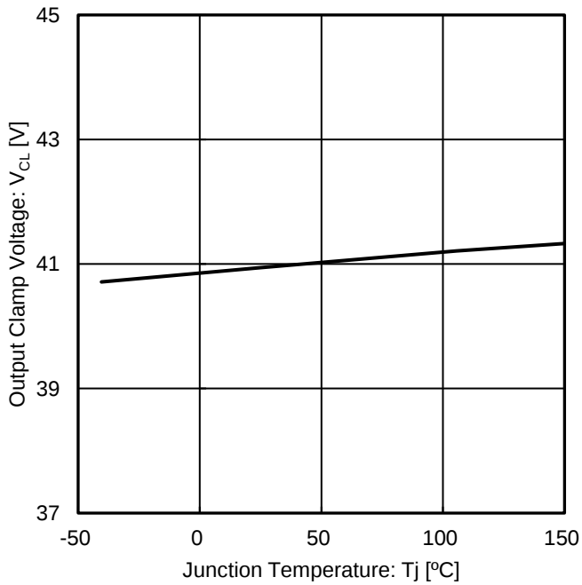
Figure 27. Output Clamp Voltage vs Junction Temperature
