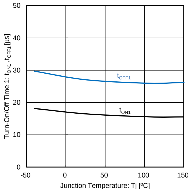
Figure 29. Turn-On/Off Time 1 vs Junction Temperature
