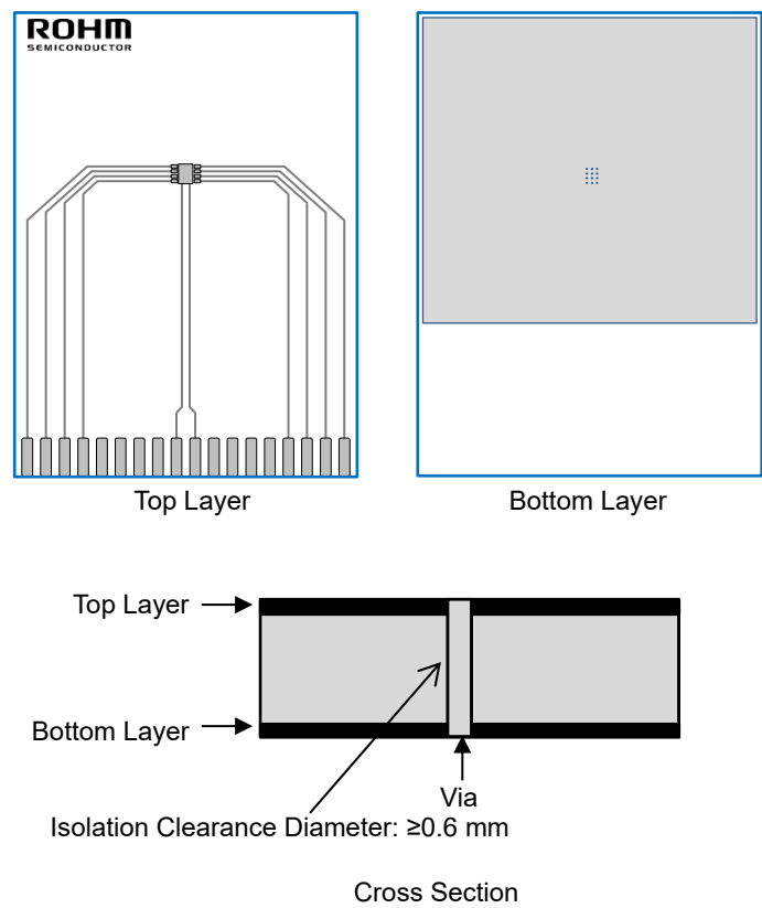
Figure 4. PCB-layout 2-layer (2s)
