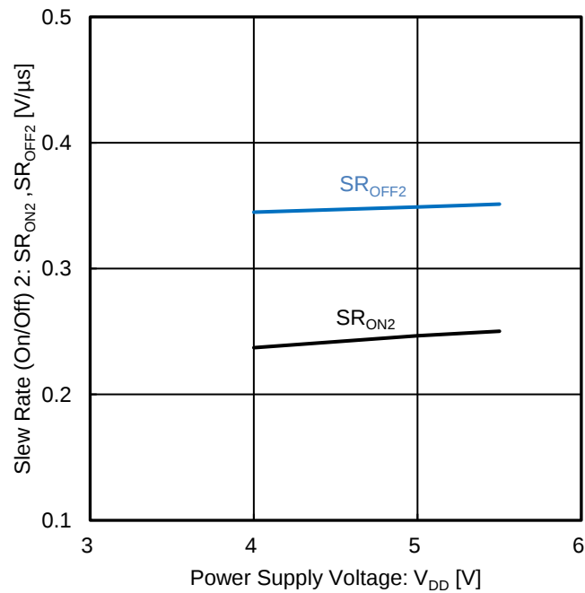
Figure 34. Slew Rate (On/Off) 2 vs Power Supply Voltage
