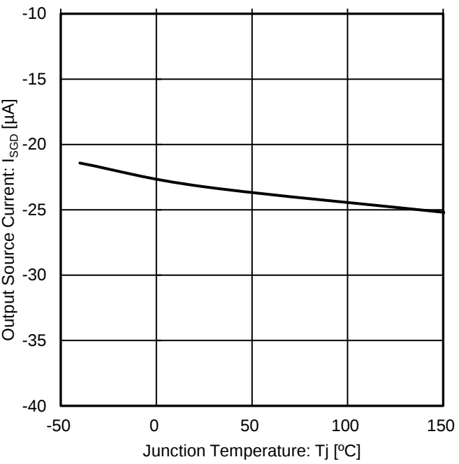
Figure 49. Output Source Current vs Junction Temperature
