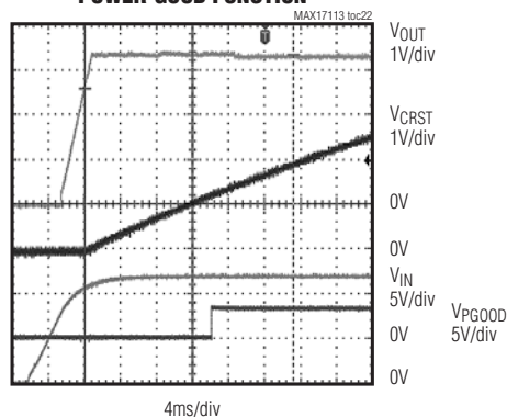
POWER-GOOD FUNCTION
