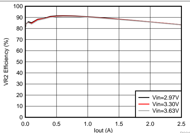
Figure 7-8. Typical Efficiency for VR2
