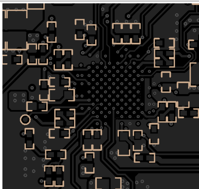
Figure 9-7. Bottom Layer ZCG Layout
