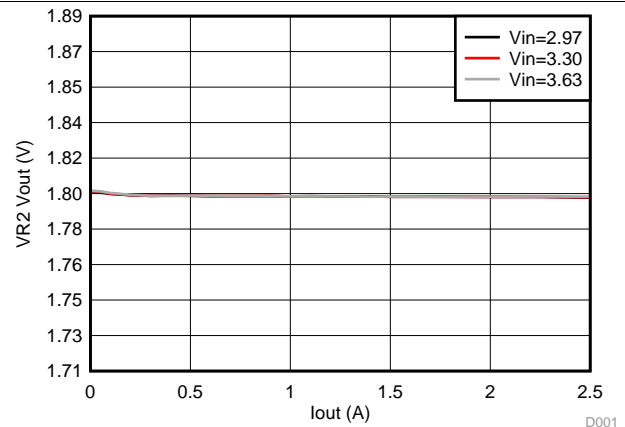
Figure 5-3. VR2 Output Voltage Load Regulation, NVDC
