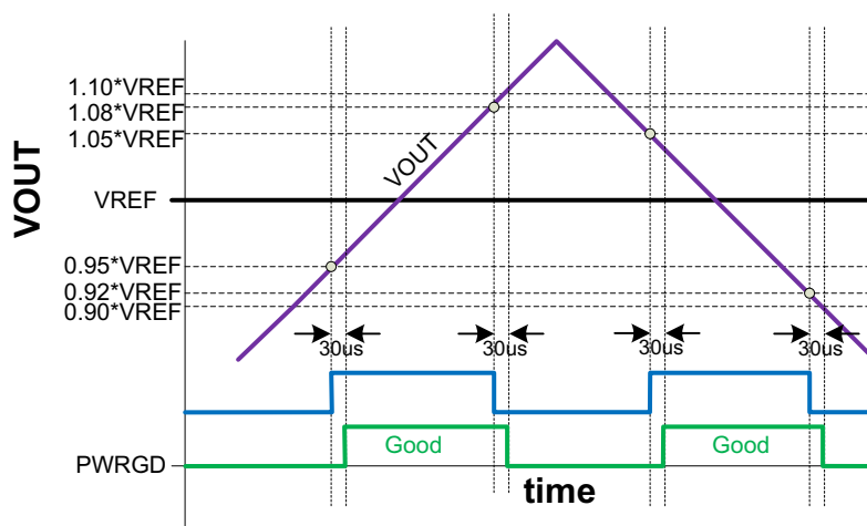
Figure 6-2. Powergood Window Comparator with Open-Drain Output
