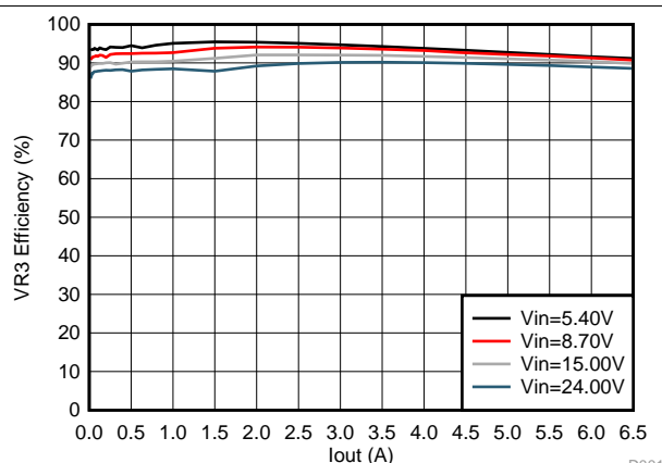
Figure 7-9. Typical Efficiency for VR3
