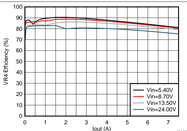
Figure 7-10. Typical Efficiency for VR4
