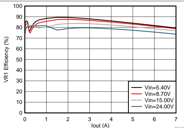
Figure 7-7. Typical Efficiency for VR1
