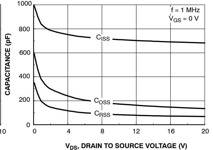
Figure 8. Capacitance Characteristics
