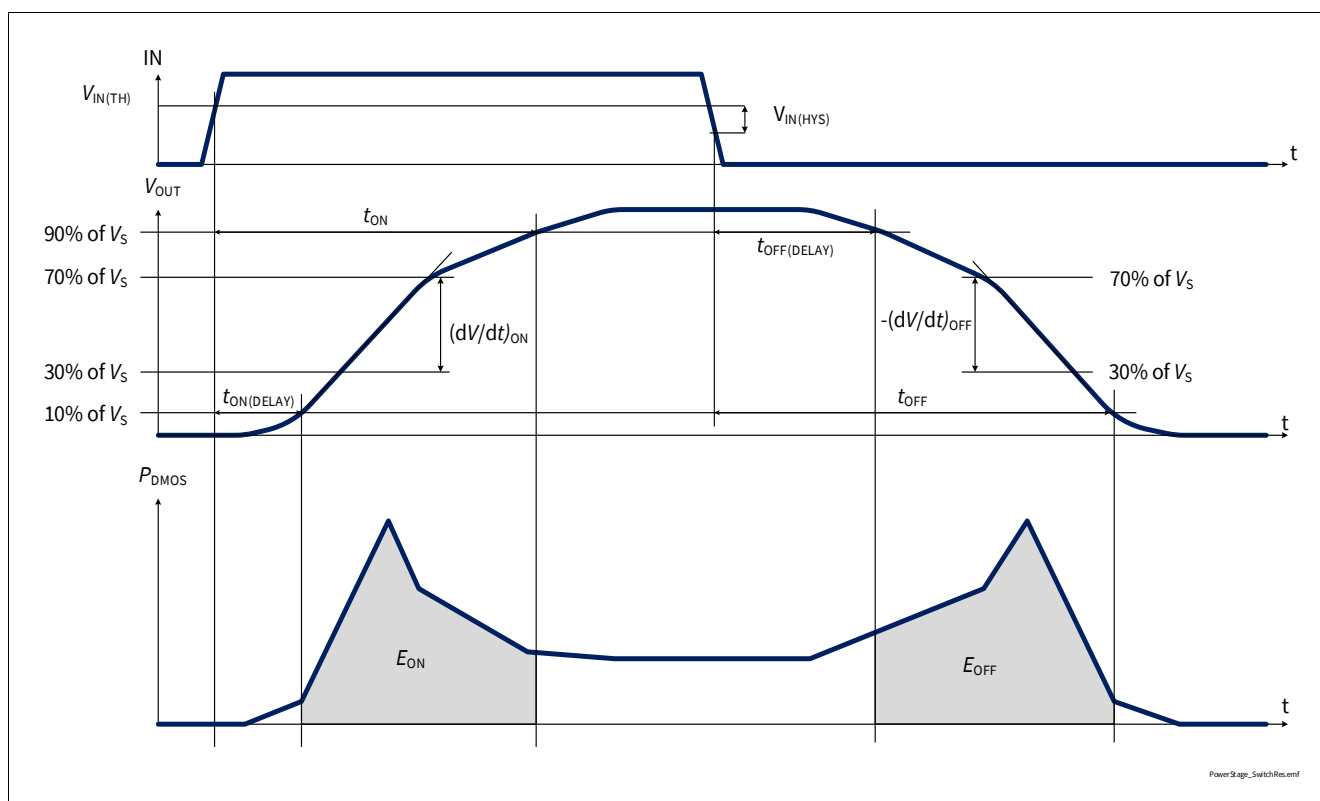
Figure 16 Switching a Resistive Load
