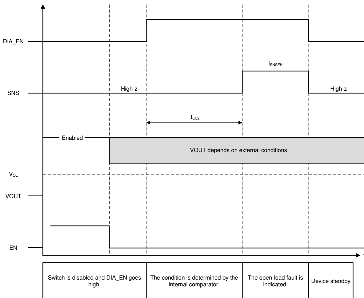
Figure 9-9. Open Load
