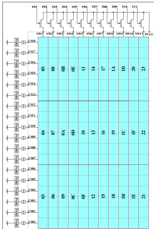
Figure 11 Open/Short Register
