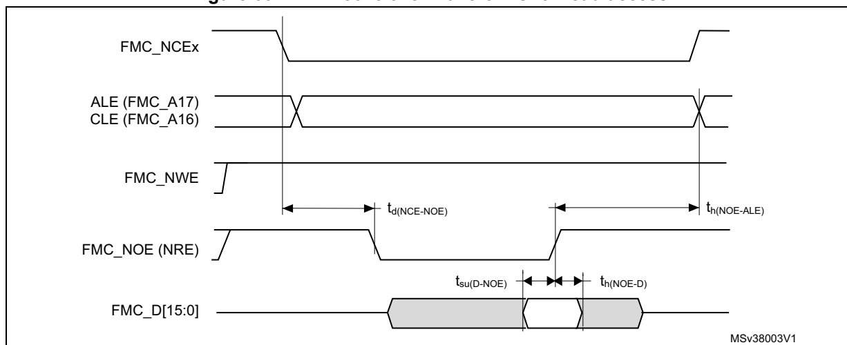
Figure 60. NAND controller waveforms for read access
