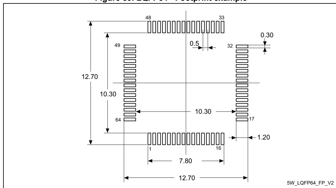
Figure 89. LQFP64 - Footprint example
