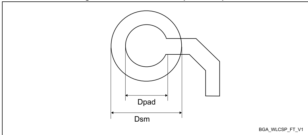
Figure 104. UFBGA169 - Footprint example
