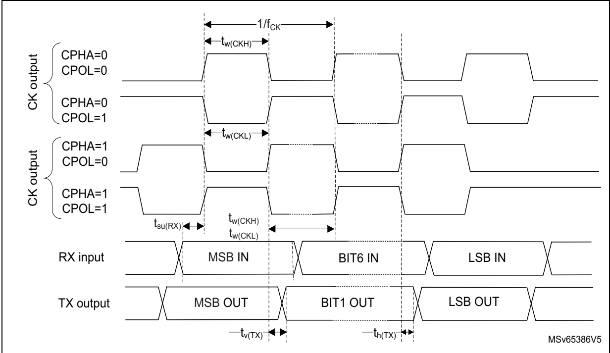
Figure 73. USART timing diagram in master mode
