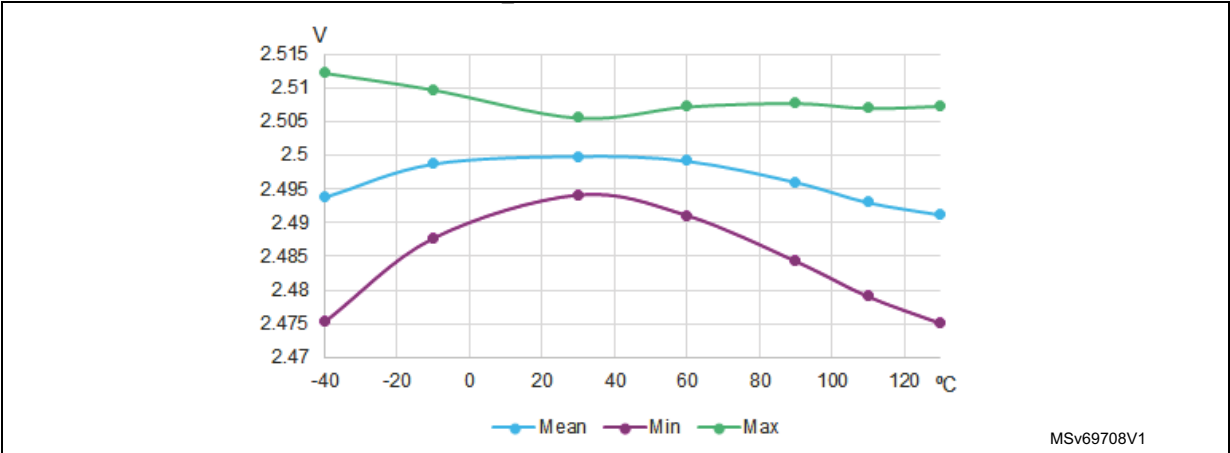
Figure 44. V_{\text{REFBUF OUT}} versus temperature (VRS = 011)
