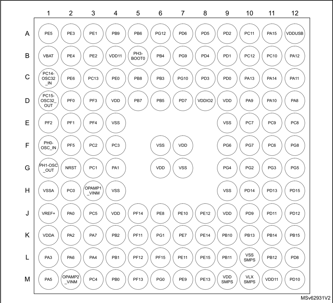
Figure 16. UFBGA132_SMPS ballout
