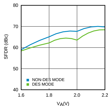
Figure 46. SFDR vs Supply Voltage (ADC12D1600)
