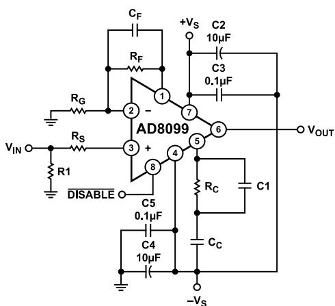
Figure 59. Wideband Noninverting Gain Configuration (SOIC)
