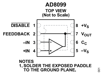
Figure 2. 8-Lead LFCSP (CP-8-13)
