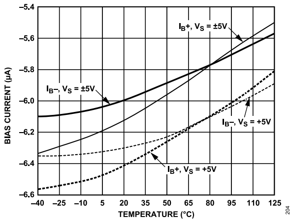
Figure 54. Input Bias Current vs. Temperature (DISABLE Pin Floating)
