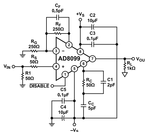
Figure 63. Amplifier Configuration for LFCSP, Gain = +2
