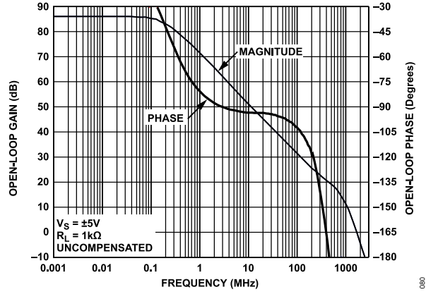
Figure 14. Open Loop Frequency Response
