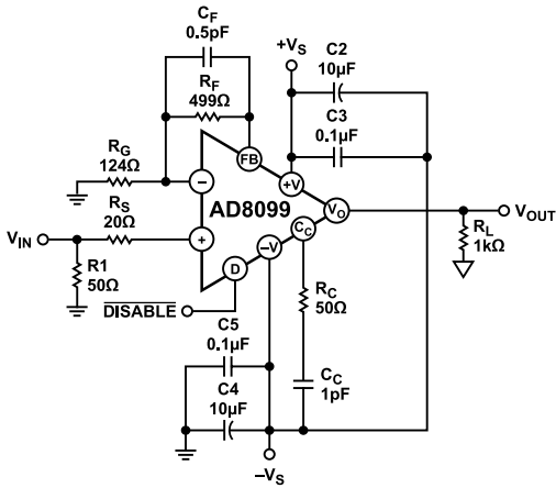
Figure 64. Amplifier Configuration for LFCSP and SOIC Package, Gain = +5
