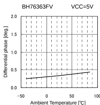
Fig.94 DP vs. Ambient Temperature
