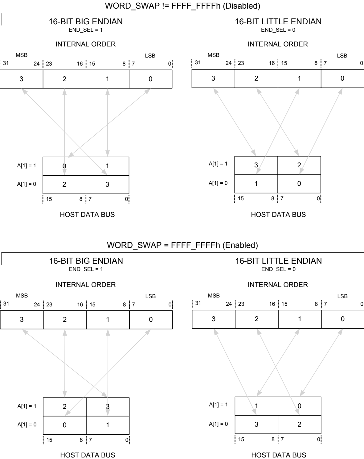
Figure 3.10 16-Bit Byte Ordering
