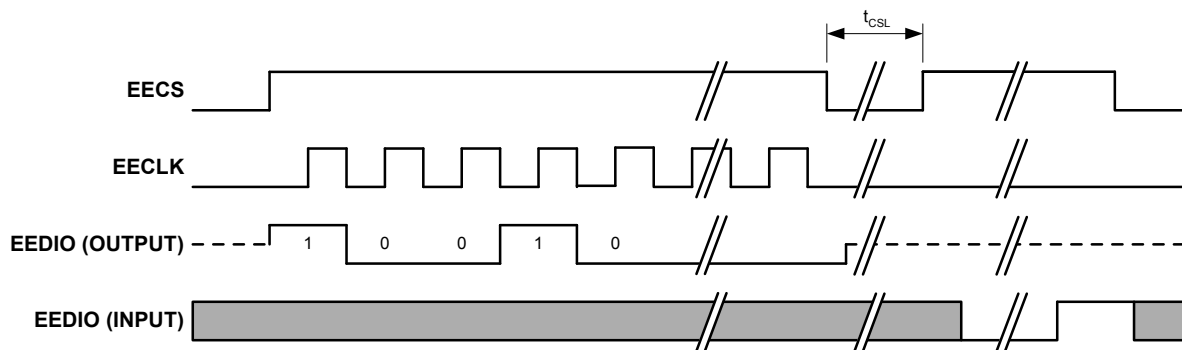
Figure 3.13 EEPROM ERAL Cycle
