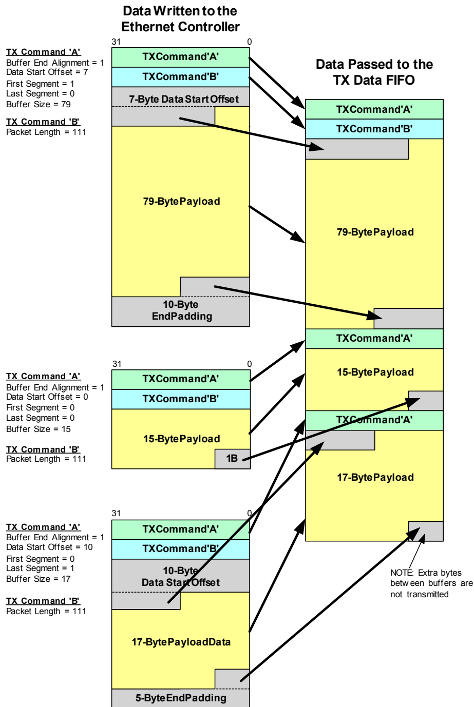
Figure 3.22 TX Example 1
