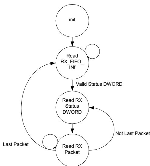
Figure 3.26 Host Receive Routine with Polling
