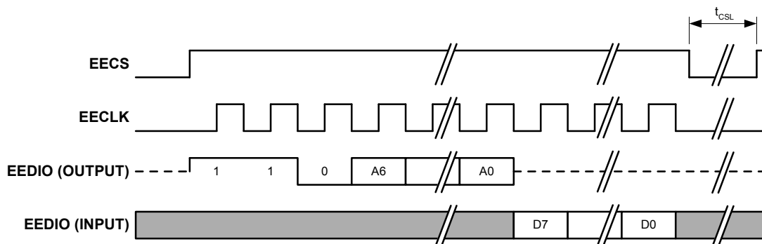
Figure 3.16 EEPROM READ Cycle
