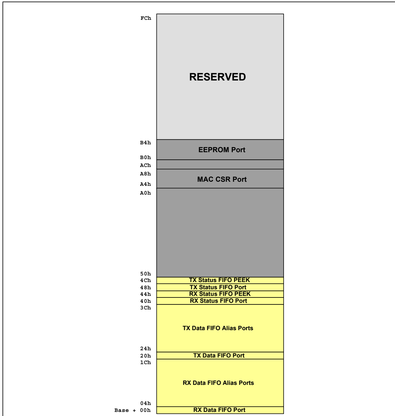
Figure 5.1 Memory Map
