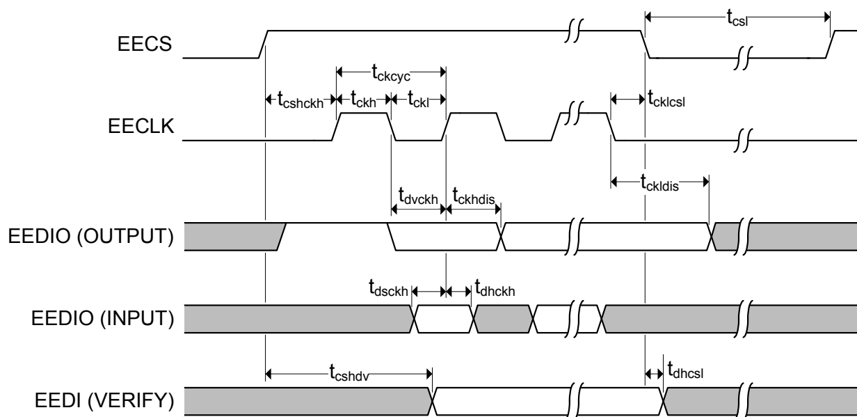
Figure 6.8 EEPROM Timing
