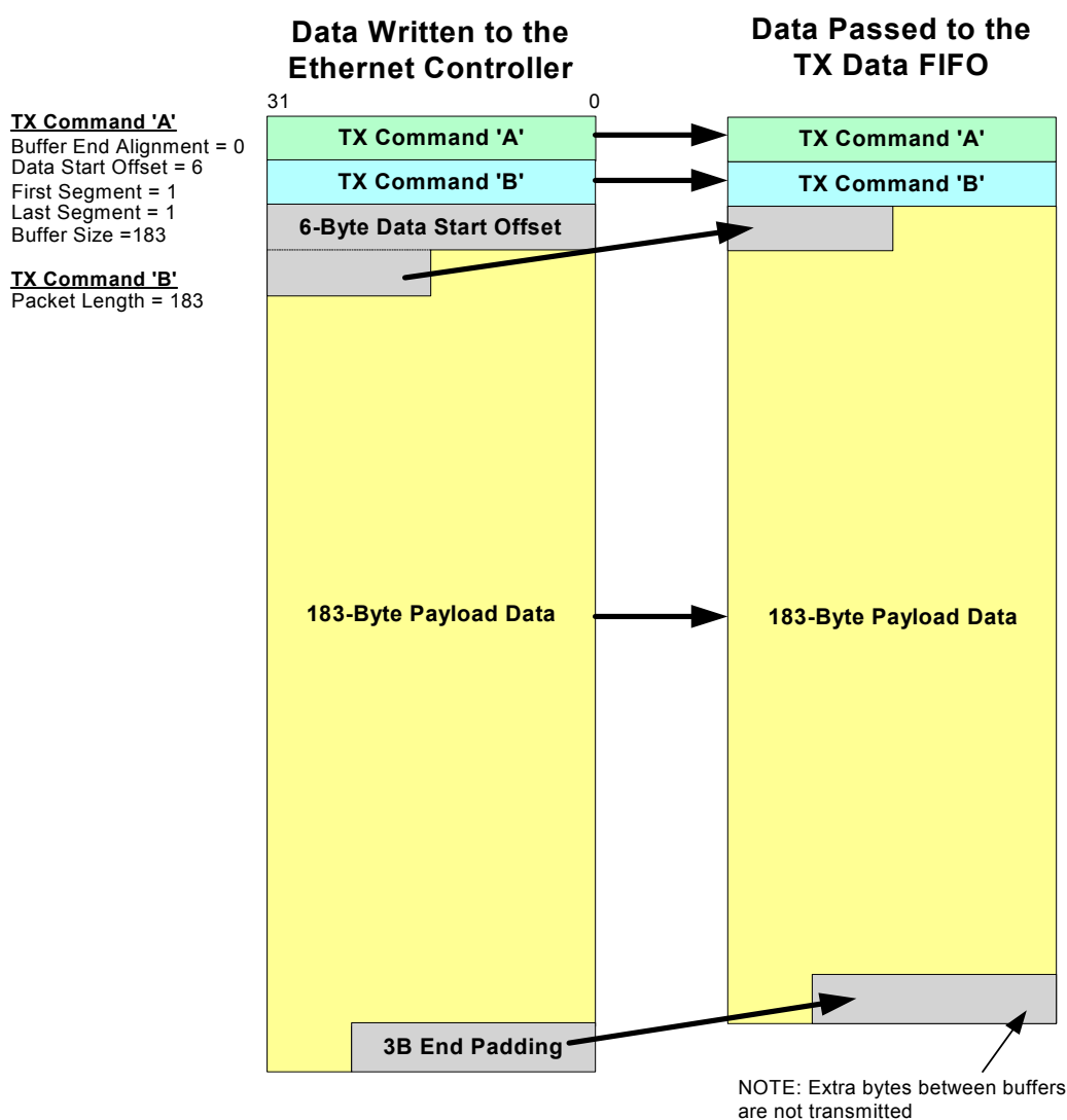
Figure 3.23 TX Example 2
