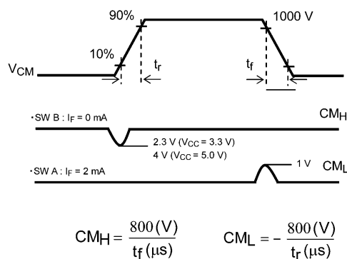
Fig. 12.1.6 Common-Mode Transient Immunity Test Circuit and Waveform
