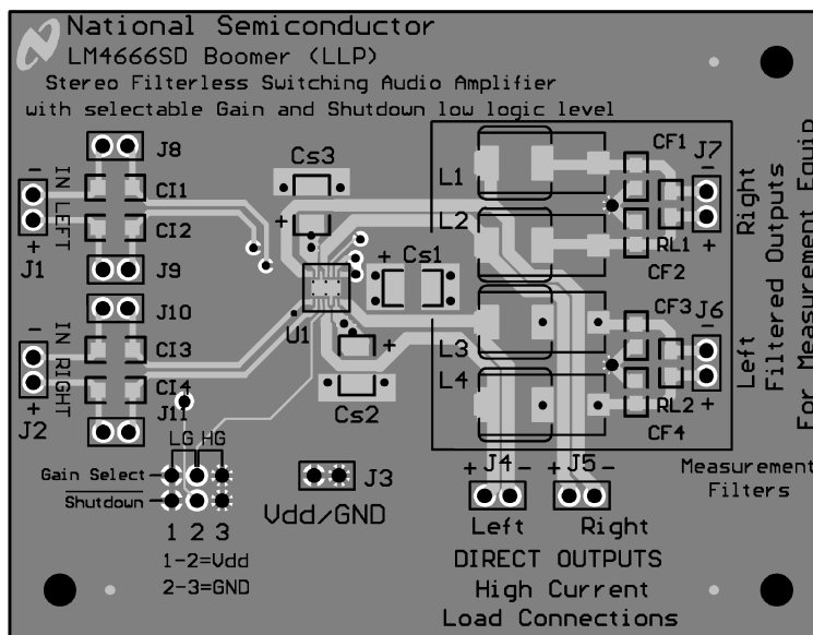
Figure 30. Silk Screen
