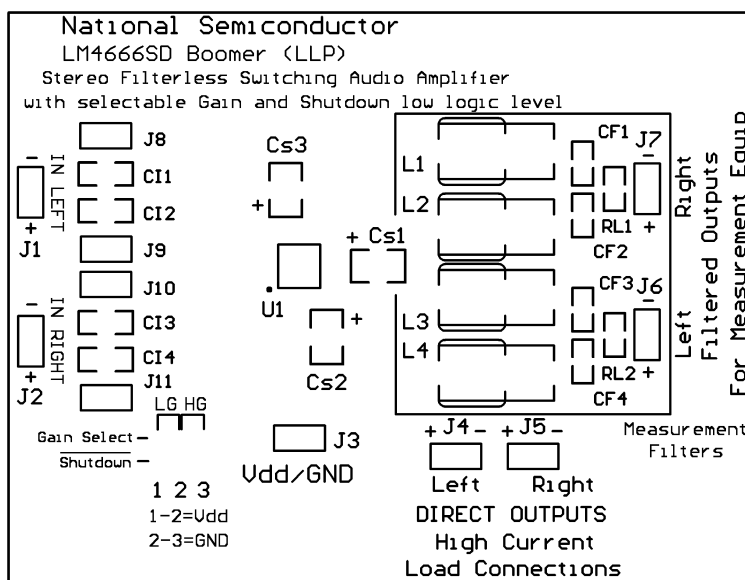
Figure 30. Silk Screen
