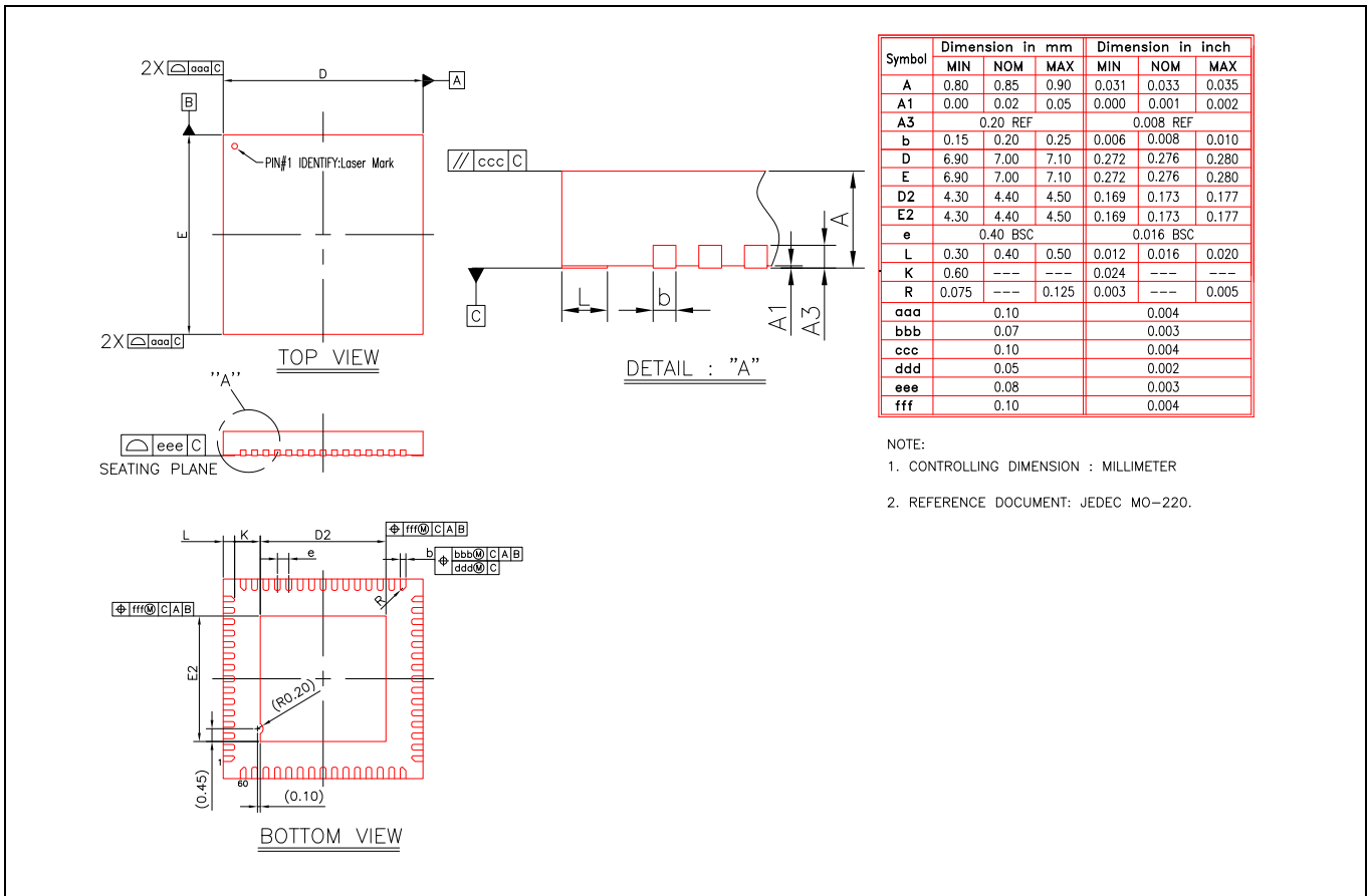
Figure 15 CYW20835 7 mm x 7 mm 60-pin QFN package
