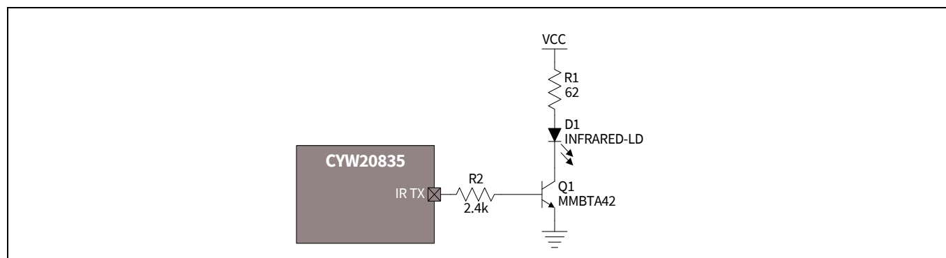
Figure 7 Infrared TX
