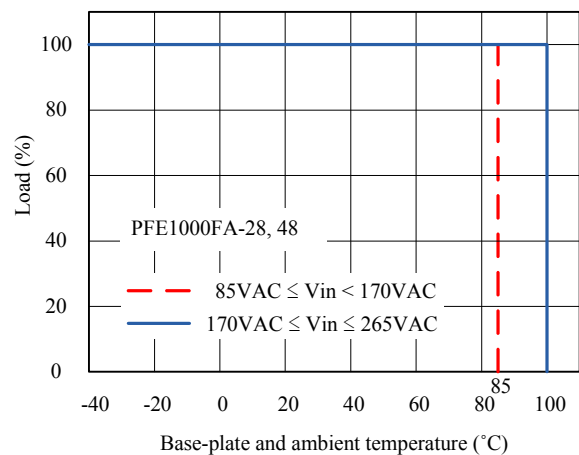
Fig.7-3-(2) PFE1000FA-28, 48 derating curve
