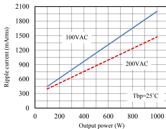
Fig.5-2 Allowable ripple current value
