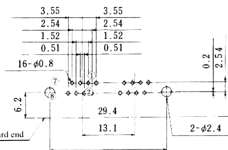
PCB mounting hole layout (Connector mounting side)
