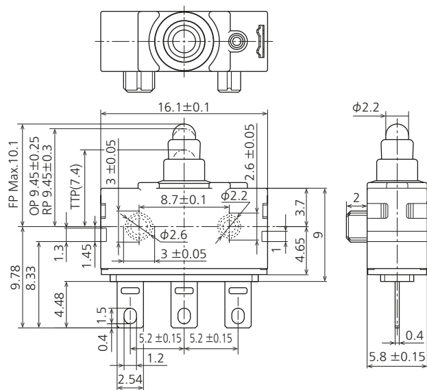
External dimensions
