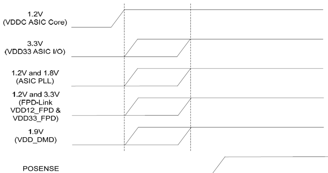
Figure 21. Initialization Timeline
