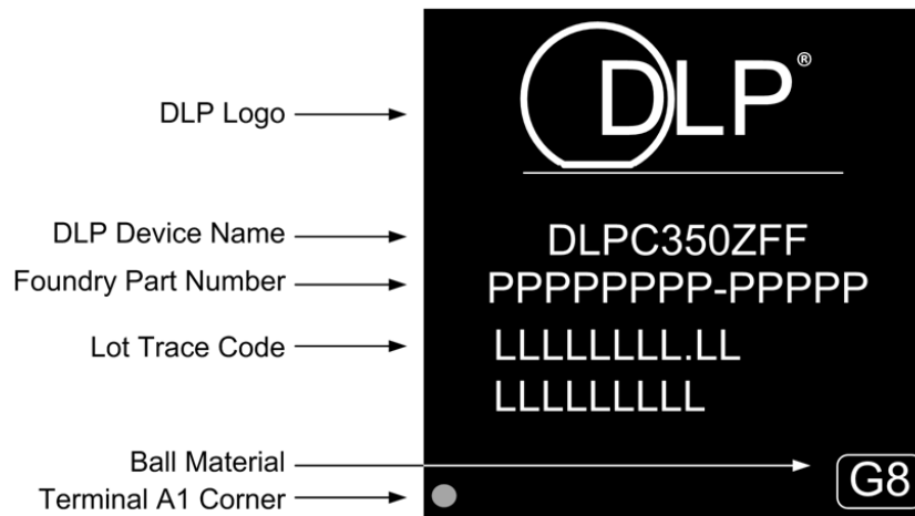
Figure 29. Device Marking
