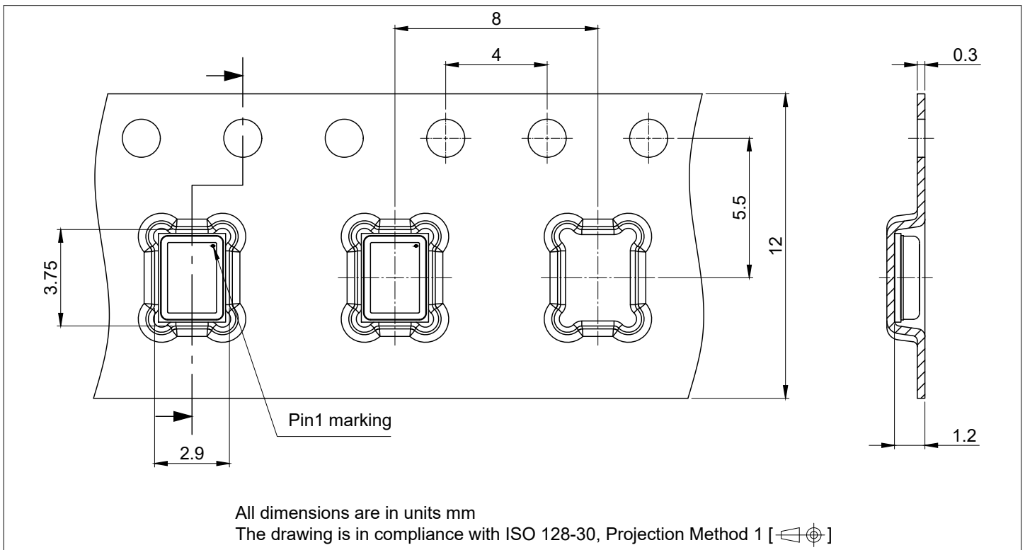
Figure 10 Tape dimensions
