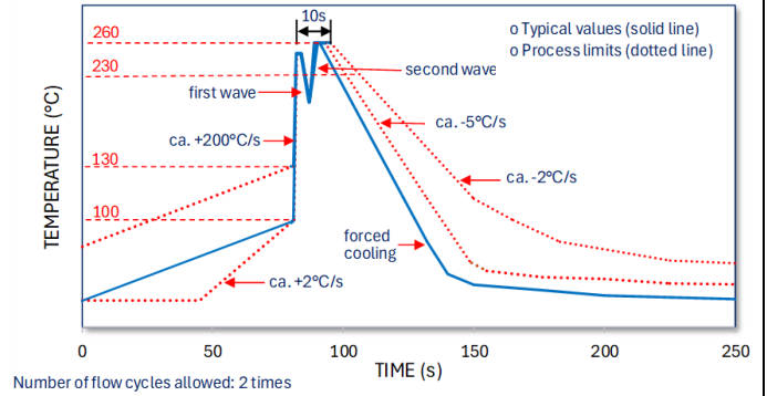
Wave Soldering Profile
